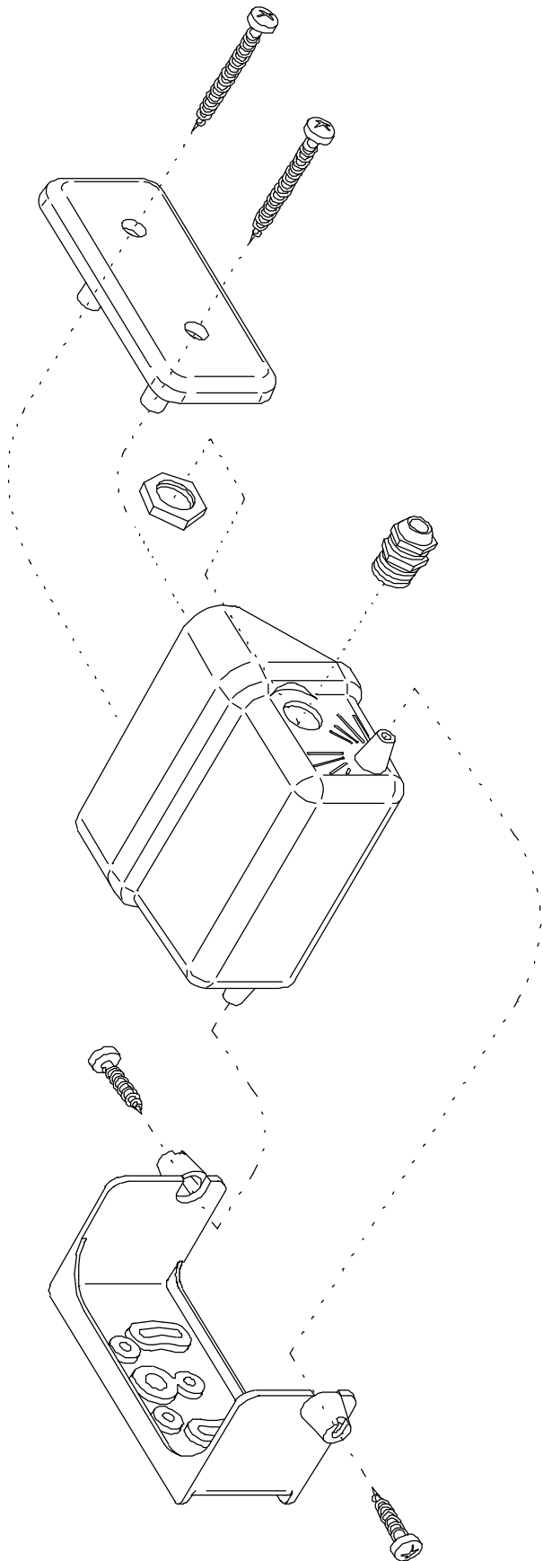
Figure 1: Magnified diagram of the housing.
