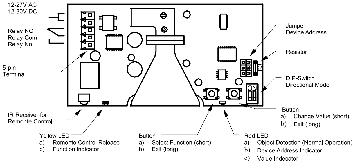
Figure 2: Operating elements on the printed board
